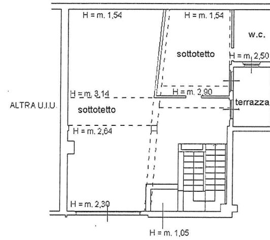
Piano 2
